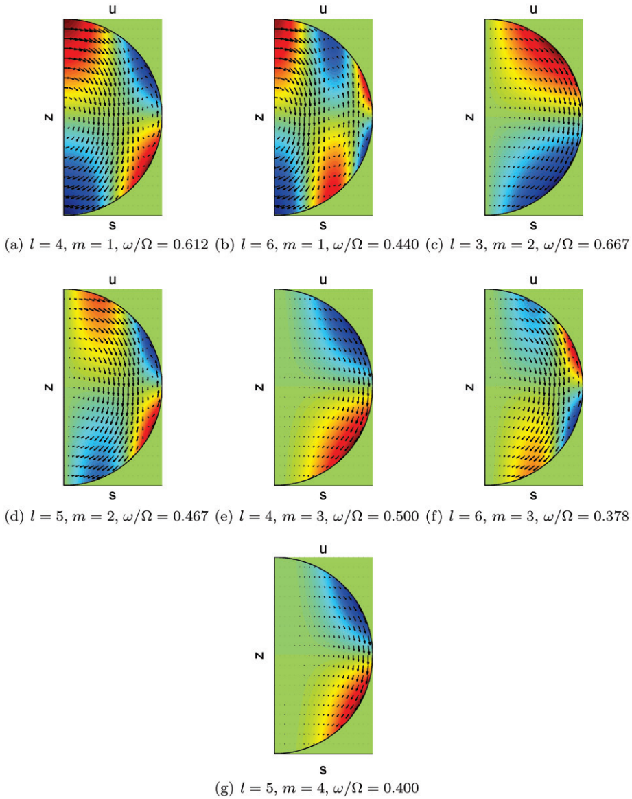
Figure 7. Velocity \mathbf{u} of the inertial modes that produce the induction shown in figures 5 and 6. Each diagram is a meridional plane in the bulk, with the axis of rotation at left and the radius normalized to 1. Arrows indicate the velocity components in the (s, z) plane and color indicates the velocity component in the \phi direction, with red for prograde flow and blue for retrograde. These plots are meant to show shape only; amplitude scales are arbitrary.
