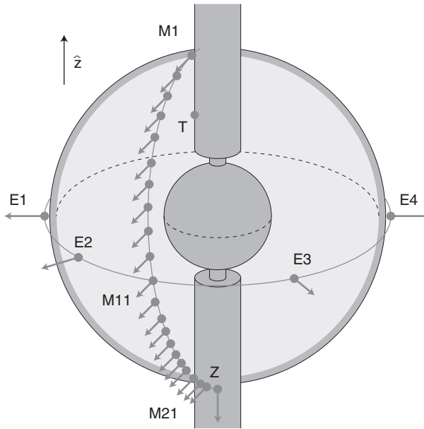
Figure 1. Diagram of the experimental setup. T marks the thermocouple; Z marks the Hall probe for measuring B_z ; labels beginning with E mark the equatorial Hall probes; and labels beginning with M mark the meridional Hall probes. The arrow at each Hall probe indicates the direction of its sensitivity. The shell between the inner and outer spheres is filled with sodium. An external field B_0 , oriented in the \hat{z} direction, is applied by two magnet coils, not shown.
