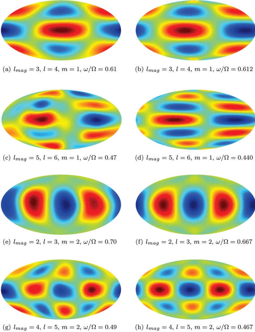
Figure 5. Induction B_s/B_0 over one revolution of the dominant pattern, shown as a Mollweide projection. Figures 5(a), 5(c), 5(e), and 5(g) show data taken under the same experimental conditions as figures 2(a), 2(b), 2(c), and 2(d), respectively. Figures 5(b), 5(d), 5(f), and 5(h) show results calculated in simulation.
