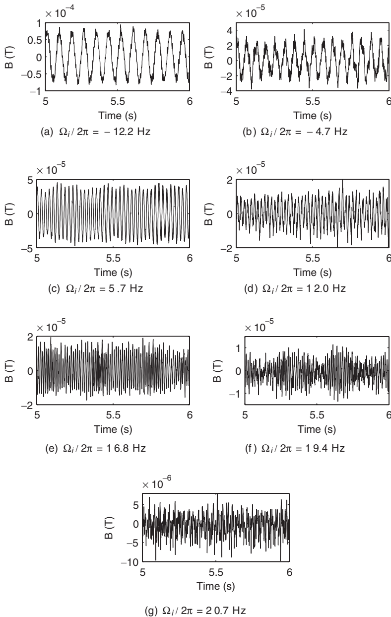
Figure 2. Typical B_s time traces at an equatorial probe. Only the oscillating component is shown, i.e., the means have been removed. For all data shown here, \Omega_o/2\pi = 29.9 Hz and B_0 = 0.015 T.
