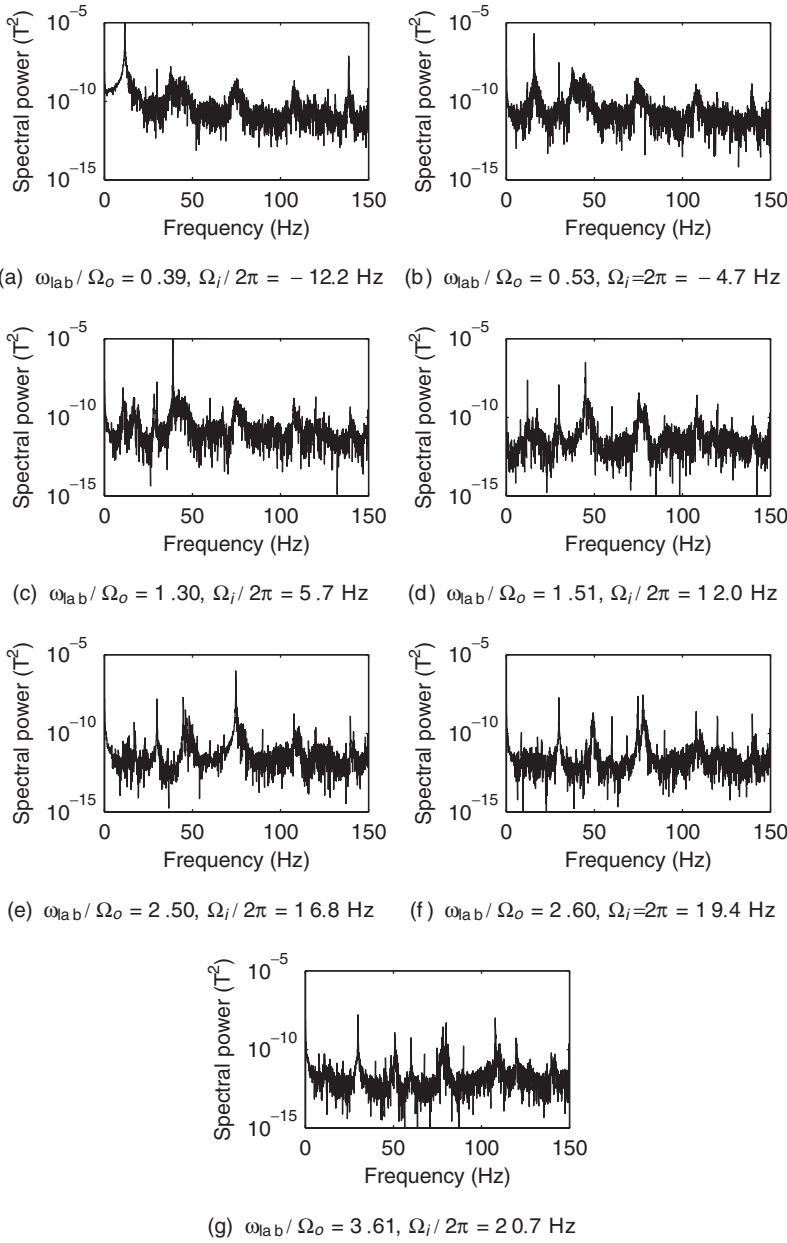
Figure 3. Power spectra of the time traces shown in figure 2. The dominant frequency in each signal is listed as \omega_{lab} / \Omega_o .
