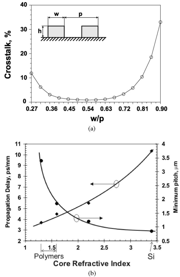
Fig. 9. Optical waveguide analysis. (a) Sketch of the modeled waveguides (inset) and the crosstalk as a function of the w/p ratio for a 10-mm polymer-core waveguide interconnect. When w/p is too small, the crosstalk is high due to a smaller mode confinement, whereas when w/p is too large, the crosstalk is high because the waveguide walls are too close. (b) The tradeoff between waveguide density and propagation delay per unit length. The graph is plotted for a 10-mm interconnect and a maximum allowed crosstalk of 20%. The height h and width w of all of the waveguides are set equal. The cladding material is assumed to have a refractive index of 1.1, and the wavelength of light is 1.3 \mu\text{m} . The optimum w/p ratio for each data point is determined separately.
