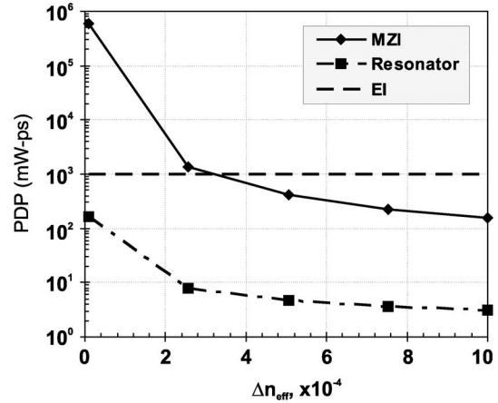
Fig. 8. Combined power-delay product of transmitter as a function of \Delta n_{\text{eff}} for the 90 nm technology node. Delay and power consumption of both the modulator and receiver circuits are included in the PDP. A series of optimized tapered inverters [15] is used to drive the modulator. The transimpedance amplifier is used to amplify the photocurrent from the detector. Additional minimum-sized inverters are used to amplify the signal to a digital level. For comparison, the dashed line describes the PDP of a 10-mm-long EI.
