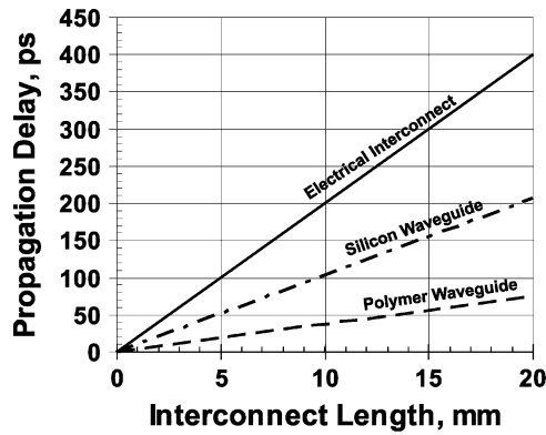
Fig. 3. Propagation delay of silicon and polymer waveguides as compared to EIs. The R-Soft full-vectorial finite-difference time-domain (FDTD) solver has been used to determine the waveguide properties. Both types of optical waveguides have a square cross section and are assumed to be surrounded by a cladding with a refractive index of 1.1. The core of the silicon waveguide is 0.34\mu\text{m} wide and has a refractive index of 3.4. The core of the polymer waveguide is 1.36\mu\text{m} wide and has a refractive index of 1.3.
