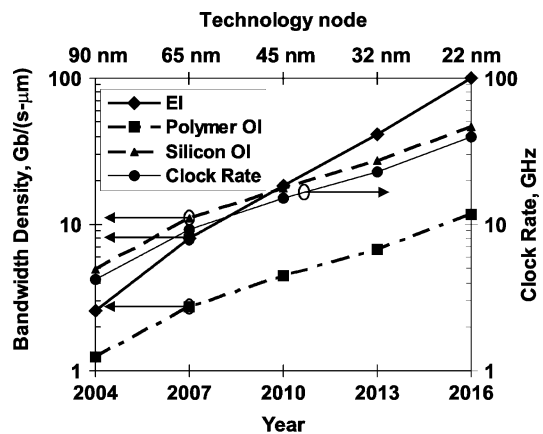
Fig. 10. Comparison of bandwidth density of electrical wires and OIs as a function of year and technology node. For reference, the thin solid line illustrates the ITRS prediction for the clock rate. Bandwidth density is an important metric, defining the information throughput of an interconnect through a unit cross section.
