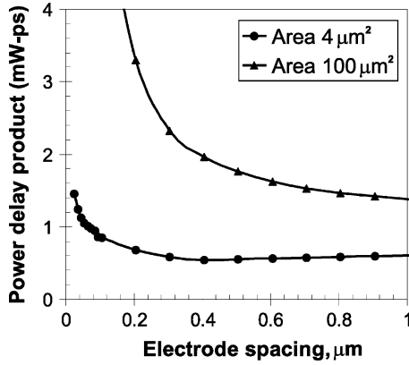
Fig. 6. Combined power-delay product for interdigitated MSM photodetector and receiver circuits.
