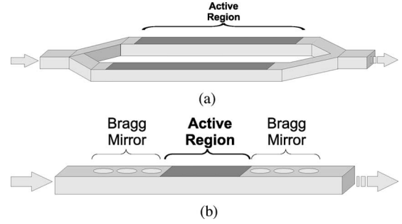
Fig. 7. Schematic of a Mach-Zehnder modulator. (a) Interferometer based. (b) Microresonator based.
