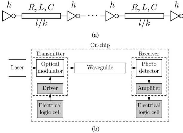
Fig. 1. (a) Circuit schematic of the EI system. (b) Block diagram of the OI system.
