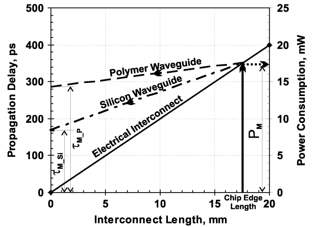
Fig. 4. Maximum conversion cost for an on-chip OI. Left axis shows the signal propagation delay and right axis the power consumption in the interconnect. \tau_{M-P} is the maximum allowed electrical-optical-electrical conversion delay in the chip edge length polymer waveguide OI, \tau_{M-Si} is the maximum allowed conversion delay in the chip edge length silicon waveguide OI, and P_M is the maximum allowed conversion power consumption in the chip edge length OI.
