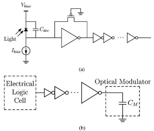
Fig. 5. Circuit schematic of (a) waveguide receiver and (b) modulator driver.
