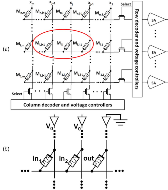
Fig. 4. MAGIC NOR gate within a crossbar array. (a) Schematic of a memristive crossbar structure. A two-input NOR gate is achieved in row i , where in_1 and in_2 are, respectively, in columns j + 1 and j , and out is in column j - 1 , as marked by an oval. (b) Schematic of a two-input NOR gate within a crossbar array. The voltage at the gateway V_0 is the applied voltage at columns j and j + 1 , whereas column j - 1 is connected to ground. Note that the schematic is identical to the figure shown in Fig. 3(a).
