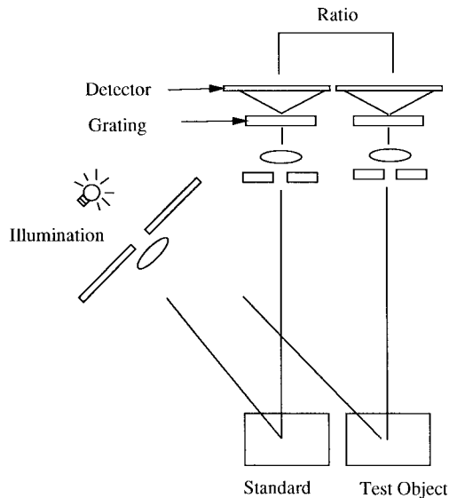
Fig. 10. Spectrophotometer measurement.
