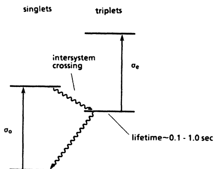
FIG. 1. Energy-level diagram showing the relevant optical interactions in fluorescein-doped boric acid glass. Due to its long luminescent lifetime, the lowest-lying triplet state acts as a trap level. \sigma_0 and \sigma_e denote the absorption cross sections of the ground and excited states, respectively.
