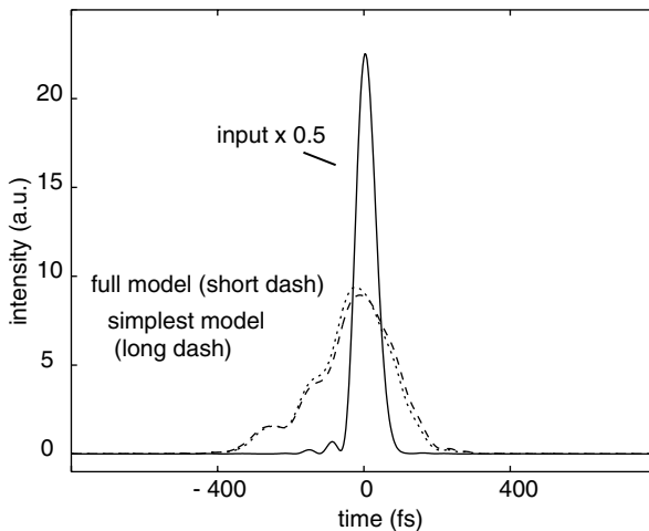
Fig. 9. Comparison of the simulated output temporal intensities obtained with the nonlinear Schrödinger equation (long dash) and with additional terms (short dash). The simulated graphs for the two different cases almost superpose.
