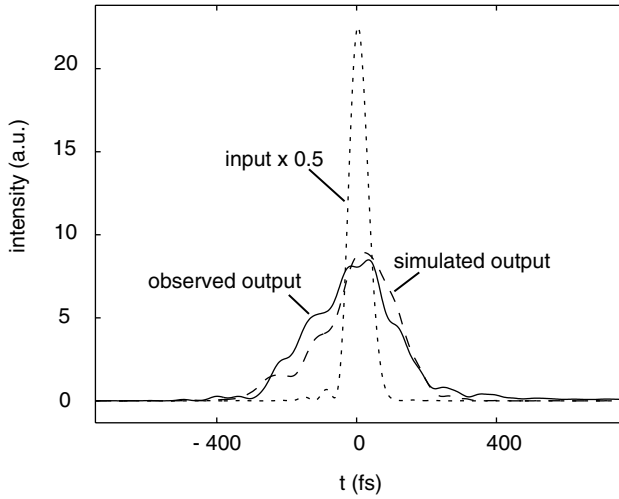
Fig. 7. Variation of the pulse temporal intensity with time as measured at the input and output of the material.
