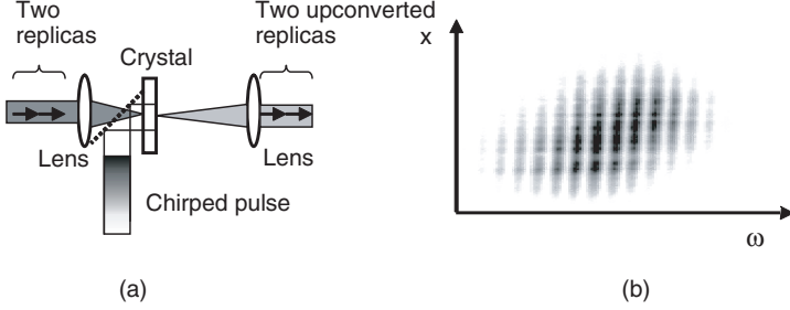
Fig. 2. (a) Generation of a spectral shear with the SPIDER technique, and (b) spatially-resolved spectral interferogram.
