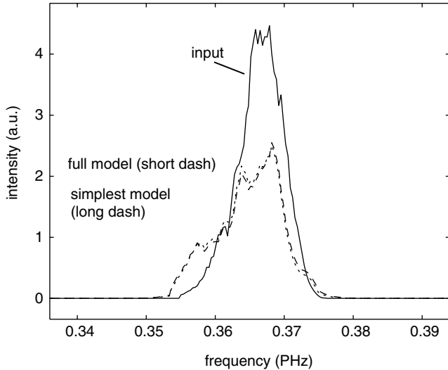
Fig. 10. Comparison of the simulated output spectral intensities obtained with the nonlinear Schrödinger equation (long dash) and with additional terms (short dash). The two simulated graphs for the two different cases almost superpose.
