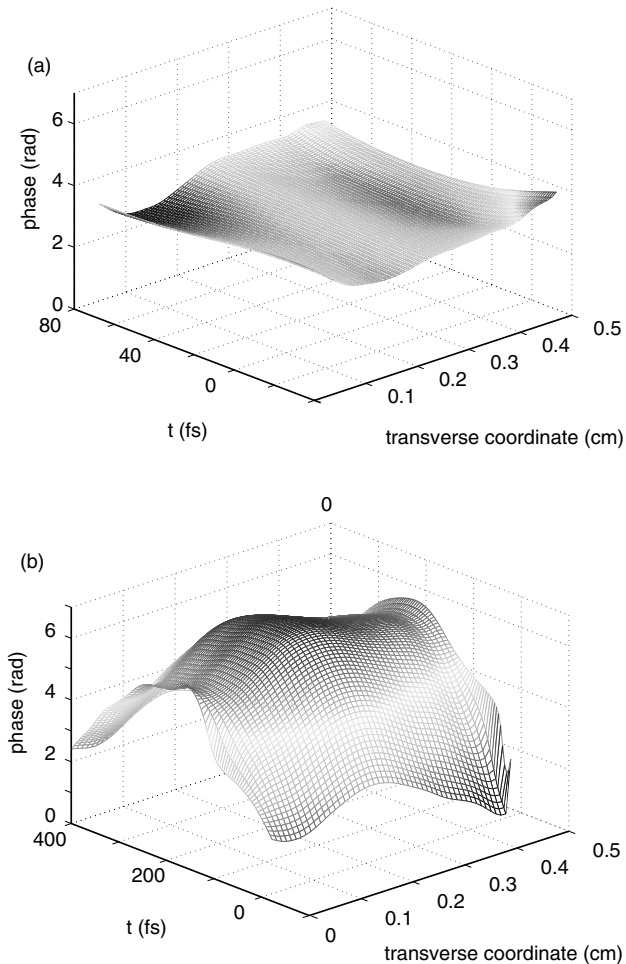
Fig. 5. Variation of the pulse phase with time and transverse coordinate at (a) the input, and (b) the output, of the SF59 glass sample as measured by spacetime SPIDER.
