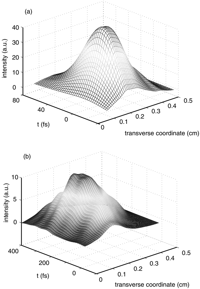
Fig. 4. Variation of the pulse intensity with time and transverse coordinate at (a) the input, and (b) the output, of the SF59 glass sample as measured by spacetime SPIDER.
