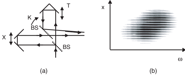
Fig. 3. (a) Generation of a spatial shear with a Michelson interferometer, and (b) spectrally-resolved spatial interferogram.
