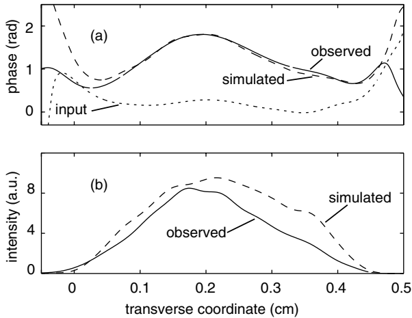
Fig. 6. (a) Input and output transverse phase variations, and (b) output intensity variations.
